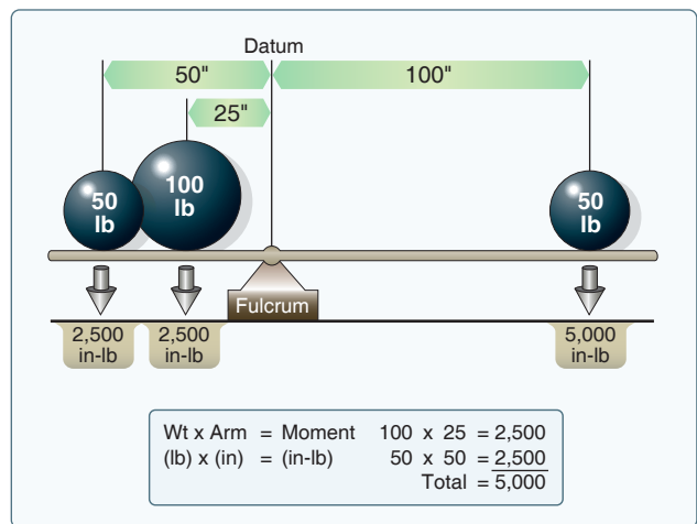
Figure 10-4. Establishing a balance.
