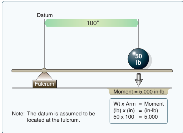
Figure 10-3. Determining moment.
