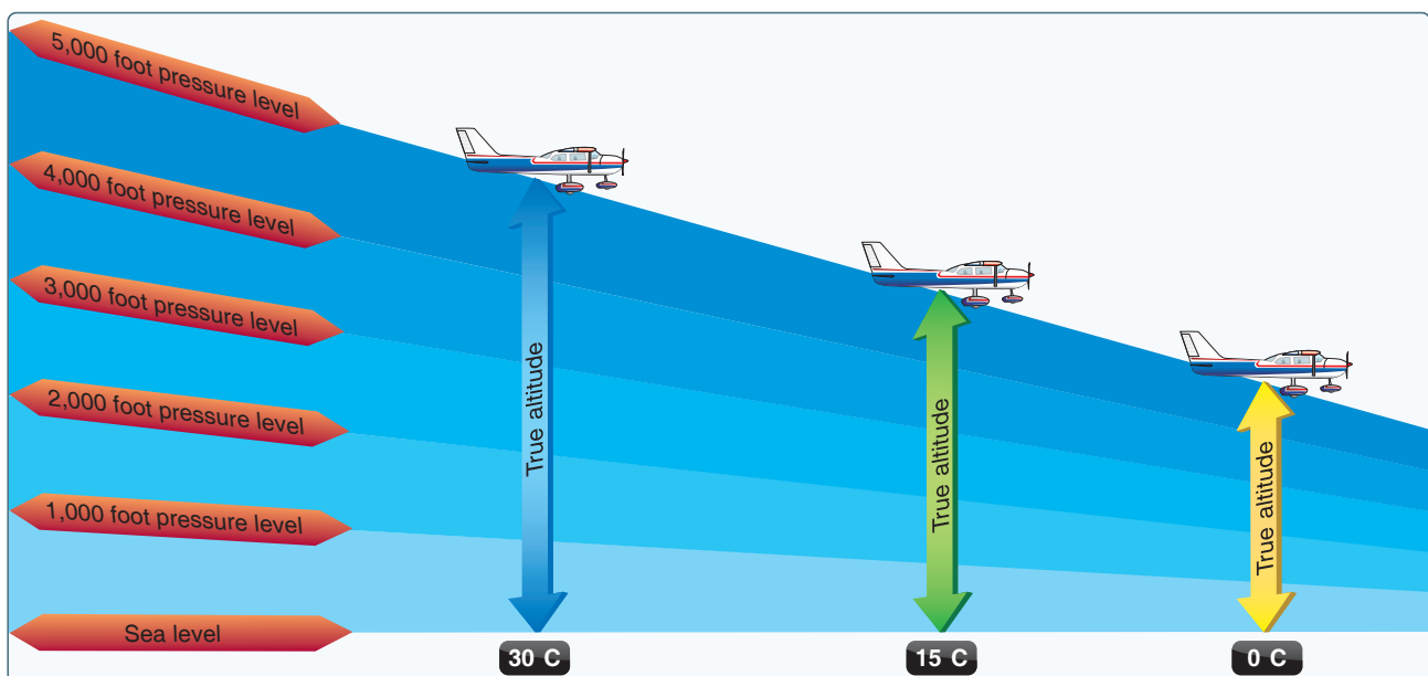
Figure 8-3. Effects of nonstandard temperature on an altimeter.
