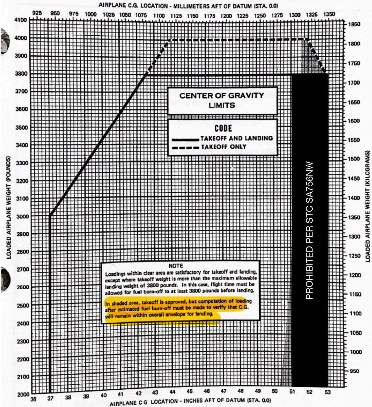
Figure 6-8. Center of Gravity Limits
