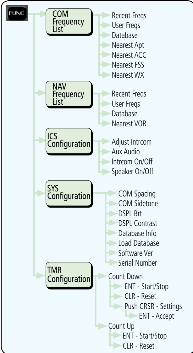
Functions Diagram
