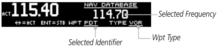
Set Selected Frequency as Active or Standby
